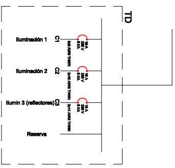
DIAGRAMA UNIFILAR
