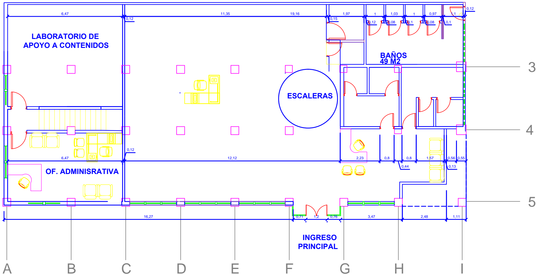
PLANTA MEZZANINE
