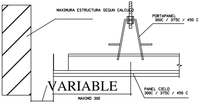
REMATE CIELO FLOTANTE
