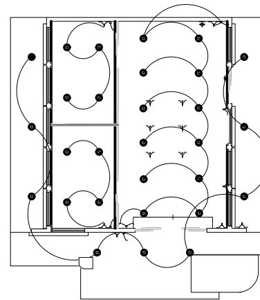
INST. ELECTRICA
