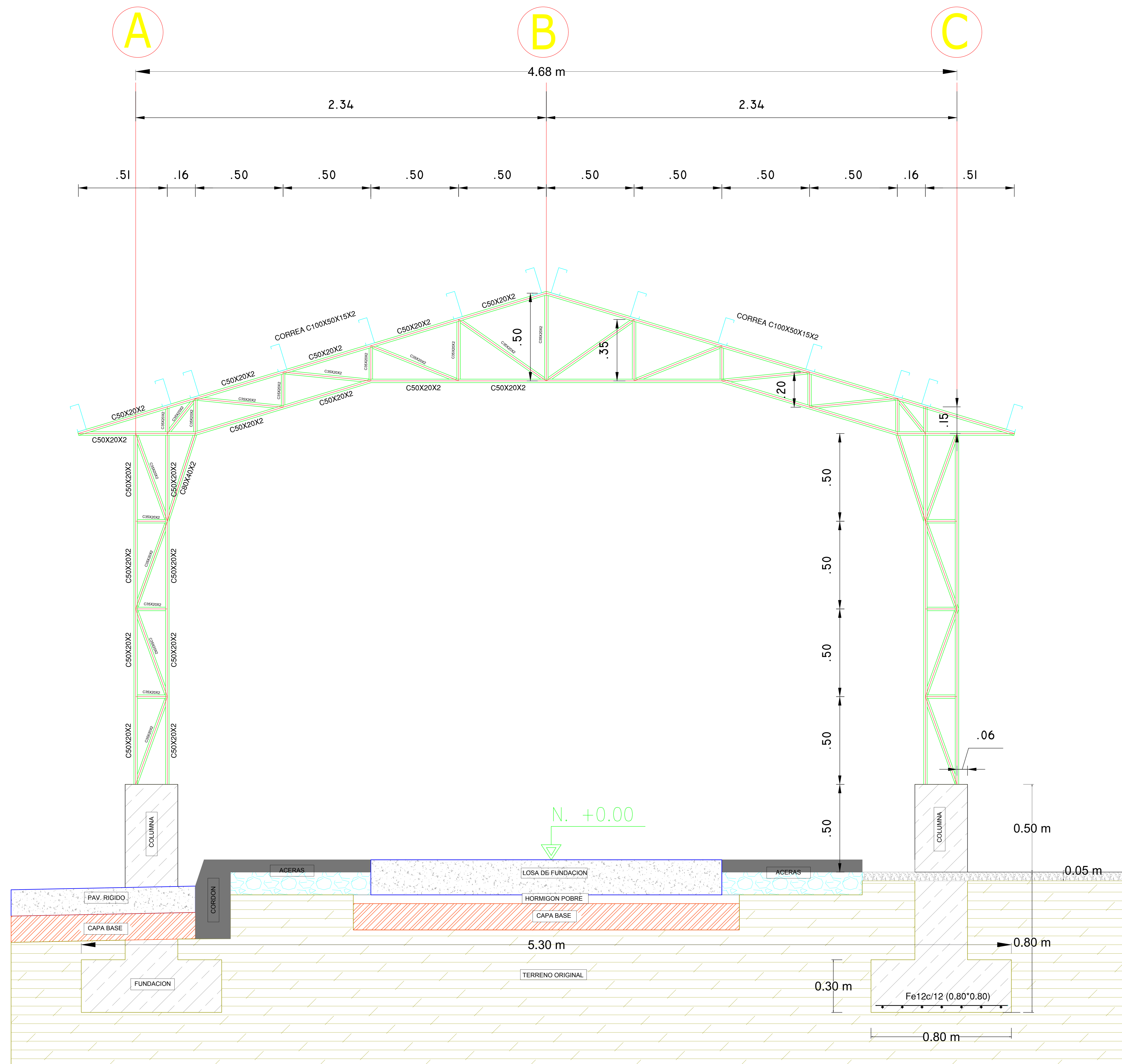
CORTE TRANSVERSAL H-H
